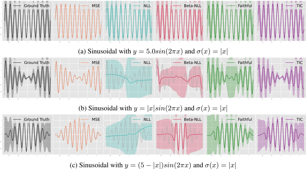
Figure 3: Synthetic-Univariate . We show that the variances learnt by mapping may not explain the randomness in the model predictions. In comparison, the Taylor Induced Covariance (TIC) performs better since it explains the (co-)variance of the predictions through the model gradient and curvature.
