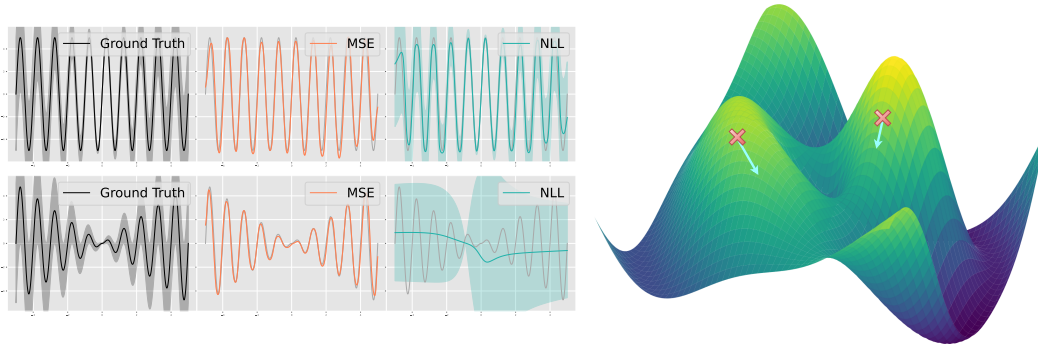
Figure 1: (Left) In the absence of supervision, \text{Cov}(\hat{\mathbf{y}}) = g_{\Theta}(\mathbf{x}) is essentially an arbitrary mapping of every \mathbf{x} to a positive definite matrix that minimizes the likelihood. As a result, \text{Cov}(\hat{\mathbf{y}}) may not truly explain the randomness in \hat{\mathbf{y}} . (Right) In contrast, the Taylor Induced Covariance (TIC) explains the randomness in \hat{\mathbf{y}} through the gradient and curvature of the mean estimator \mathbf{y} = f_{\theta}(\mathbf{x}) . Intuitively, the gradient and curvature quantify the variation in the prediction within an \epsilon -neighborhood of \mathbf{x} .
