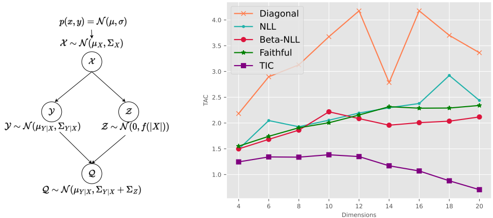
Figure 4: Synthetic-Multivariate . (Left) Experiment Design: We simulate correlated input-target variables with heteroscedastic covariance. (Right) Results: We plot the Task Agnostic Correlations (TAC) metric (y-axis) for all methods from dimensions 4 to 20 (x-axis). We show that the gap between the Taylor Induced Covariance (TIC) and other baselines widens with increasing dimensionality.
