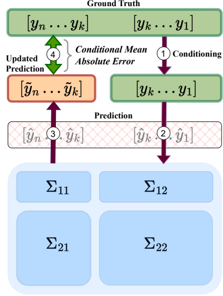
Figure 2: We propose TAC: Task Agnostic Correlations as a metric to assess the quality of covariance estimation. Given the ground truths, predicted mean and the predicted covariance matrix, TAC quantifies the improvement in the predicted mean given partial observations of the ground truth. TAC uses conditioning of the normal distribution as a direct measure to assess the quality of covariance.
